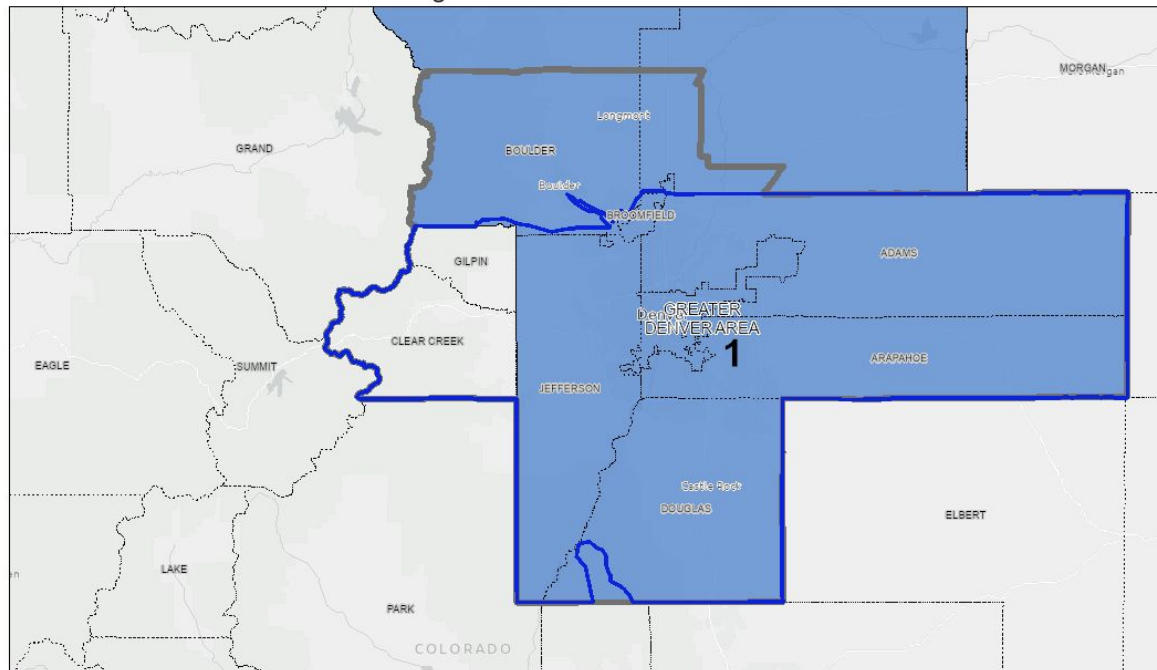
Region 1 Ozone Nonattainment
