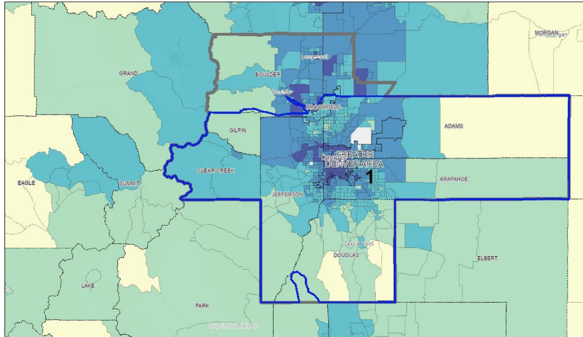
Region 1 Levels of Air Pollutants: Air Quality Measures
